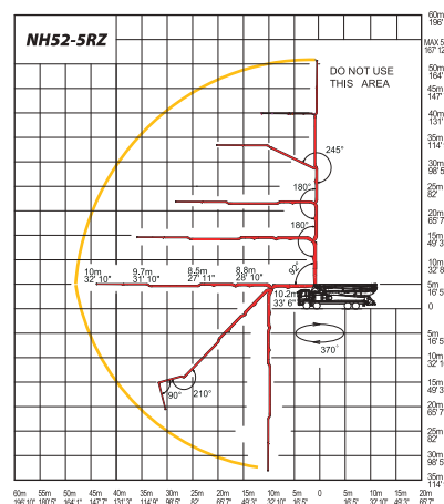
Working Range
