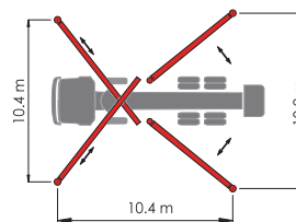
Out Rigger Diagram
