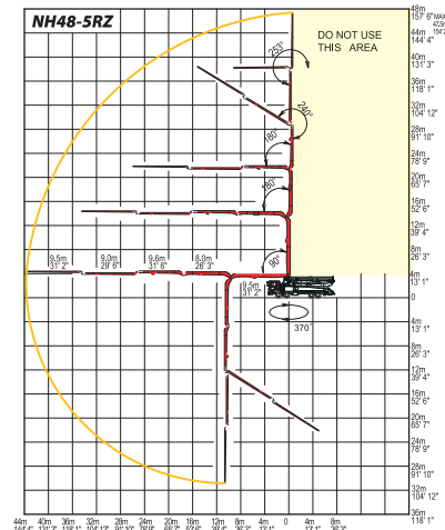
Working Range
