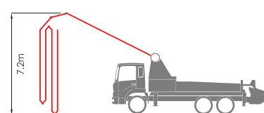
Unfolding height
