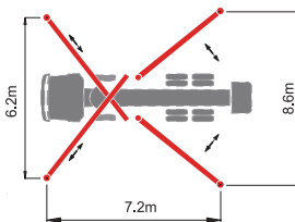
Pump Specification
